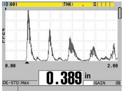
Outdoor display setting, A-scan mode
