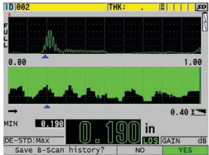
Indoor display setting, B-scan mode
